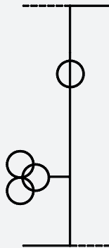
Type MME 365 Bus Riser with Metering Unit
