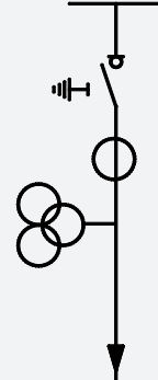
Type MME 363 Line with Metering Unit
